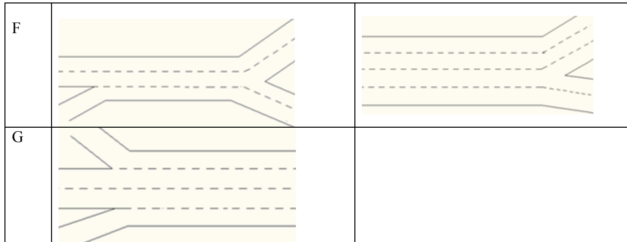
Fig. 1. Types of lane-ramp configurations found in the study area
