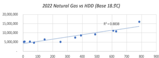
Figure 3: Natural Gas vs HDD
