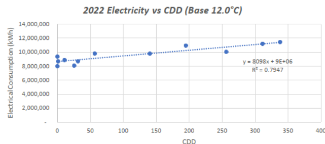
Figure 2: Electricity vs CDD
