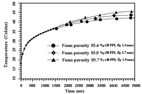
FIG. 7. Temperature-time history for different pore size foams.
