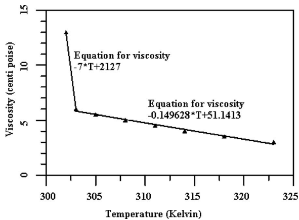
FIG. 1. Variation of pure wax viscosity with temperature.
