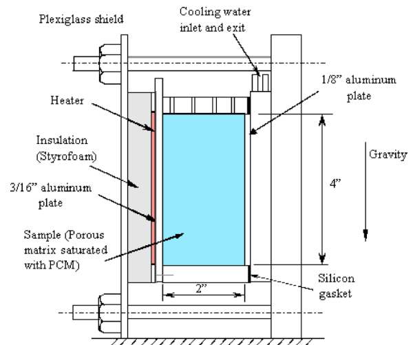
FIG. 2. (Color online) Experimental setup for phase change analysis of composite samples (front view).
