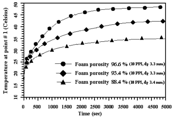
FIG. 5. Heater temperature-time history for different porosity Al foam.
