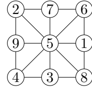
(B) A magic square viewed as a magic polygon
