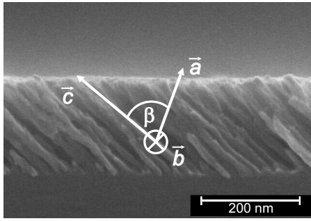
FIG. 1. SEM micrograph of slanted Ti nanocolumns grown on a Si substrate. The overlaid coordinate system indicates the orientation of the monoclinic biaxial system with its internal c -axis along the nanocolumns and b -axis parallel to the film interface. The angle \beta between axes a and c is 67.5^\circ .
