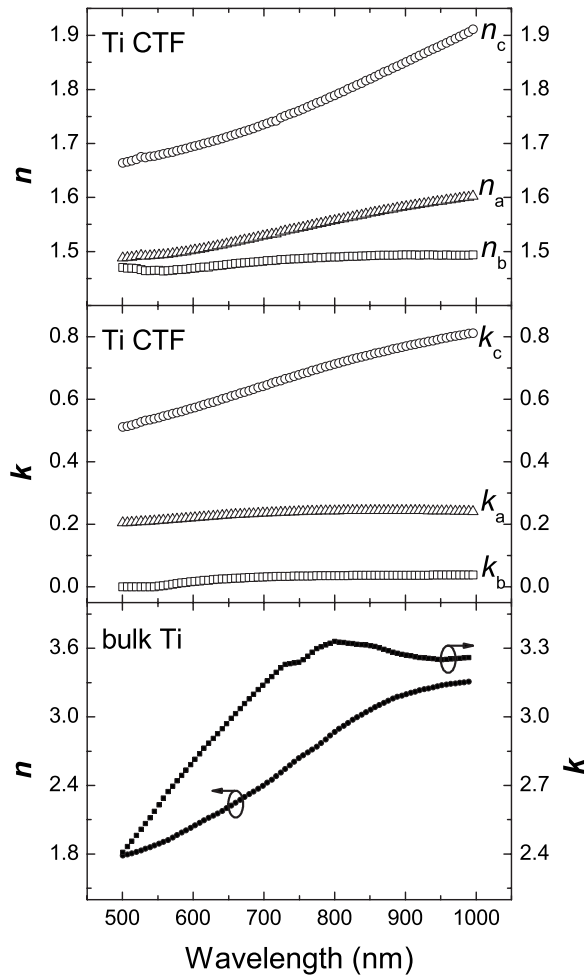
FIG. 3. Monoclinic optical constants n_a , n_b , n_c and k_a , k_b , k_c obtained from the best-model calculation for Ti CTF sample in Fig. 1, and bulk Ti optical constants for comparison.
