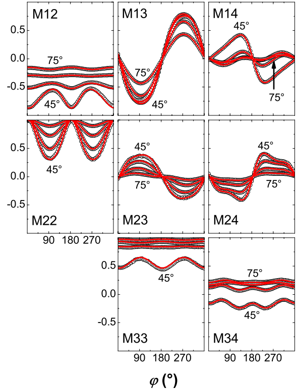
FIG. 2. (Color online) Exemplary experimental (symbols) and best-match (solid lines) calculated GE data vs sample azimuth \varphi and angle of incidence \Phi_a at \lambda = 850 nm.
